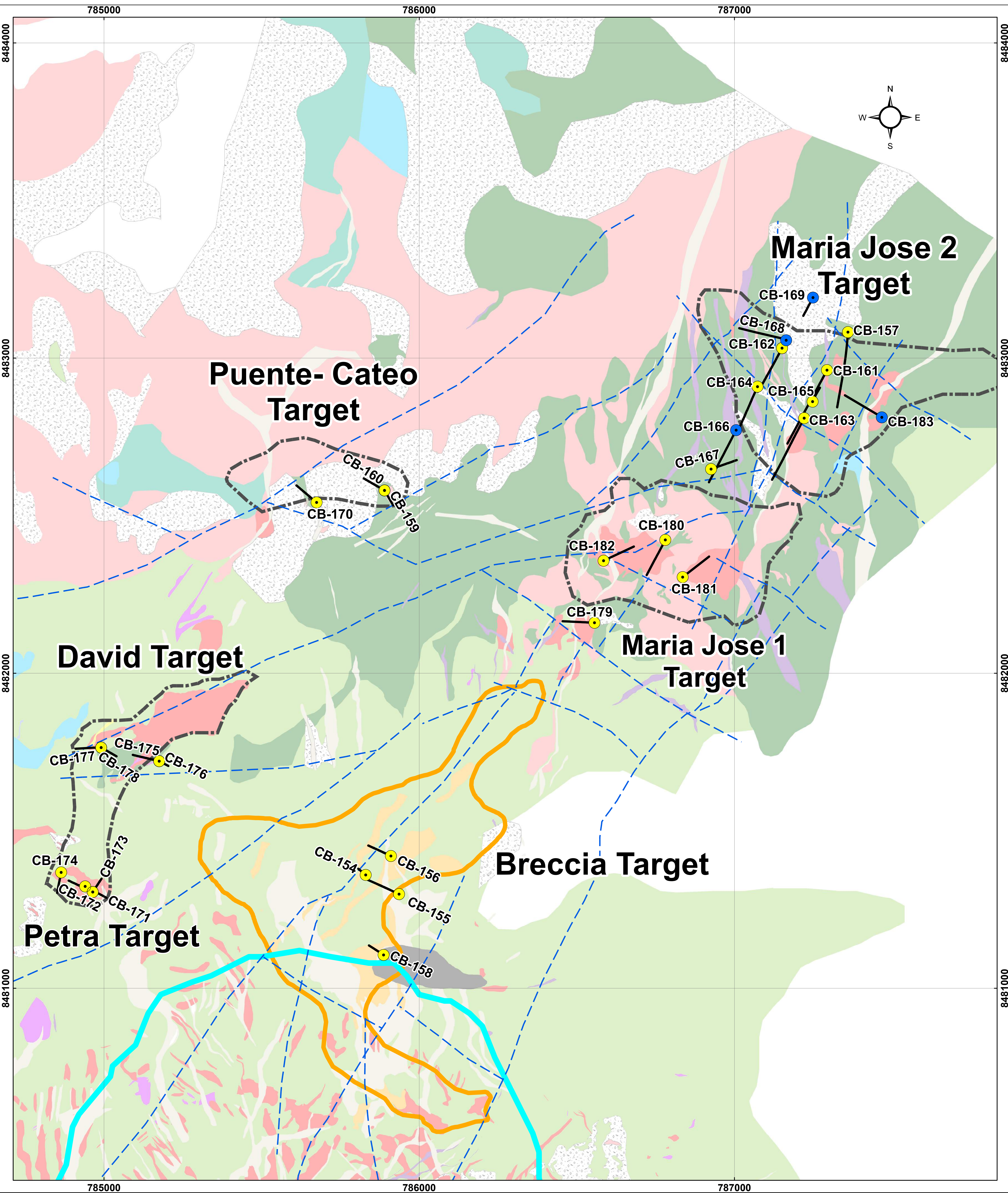
CLUSTER 1 TARGETS - GEOLOGY MAP 0 250 500 1:5,000 m
